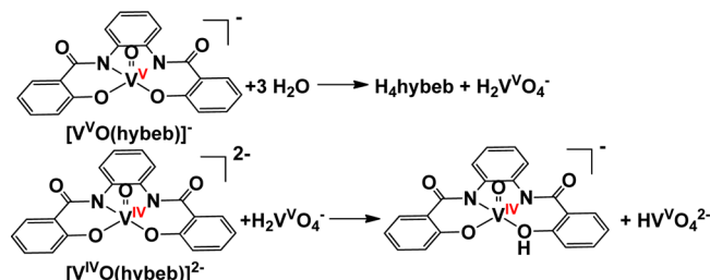
Scheme 2. Possible Mechanism of the Protonation of the Complex Anion [\text{V}^{\text{IV}}\text{O}(\text{hybeb})]^{2-} Leading to [\text{V}^{\text{IV}}\text{O}(\text{Hhybeb})]^{-} through Hydrolysis of [\text{V}^{\text{IV}}\text{O}(\text{hybeb})]^{-}
