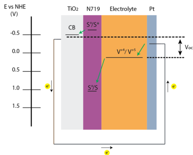
Figure 8. Redox potential for (\text{Ph}_4\text{P})_2[\text{V}^{\text{IV}}\text{O}(\text{hybeb})] and (\text{Ph}_4\text{P})-[\text{V}^{\text{V}}\text{O}(\text{hybeb})] mediators in relation to the energy levels of the dye/TiO 2 photoanode.
